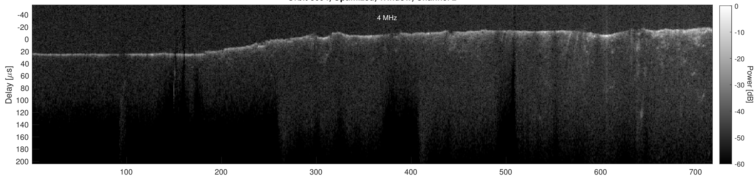
Orbit 3094, Cluttergram
