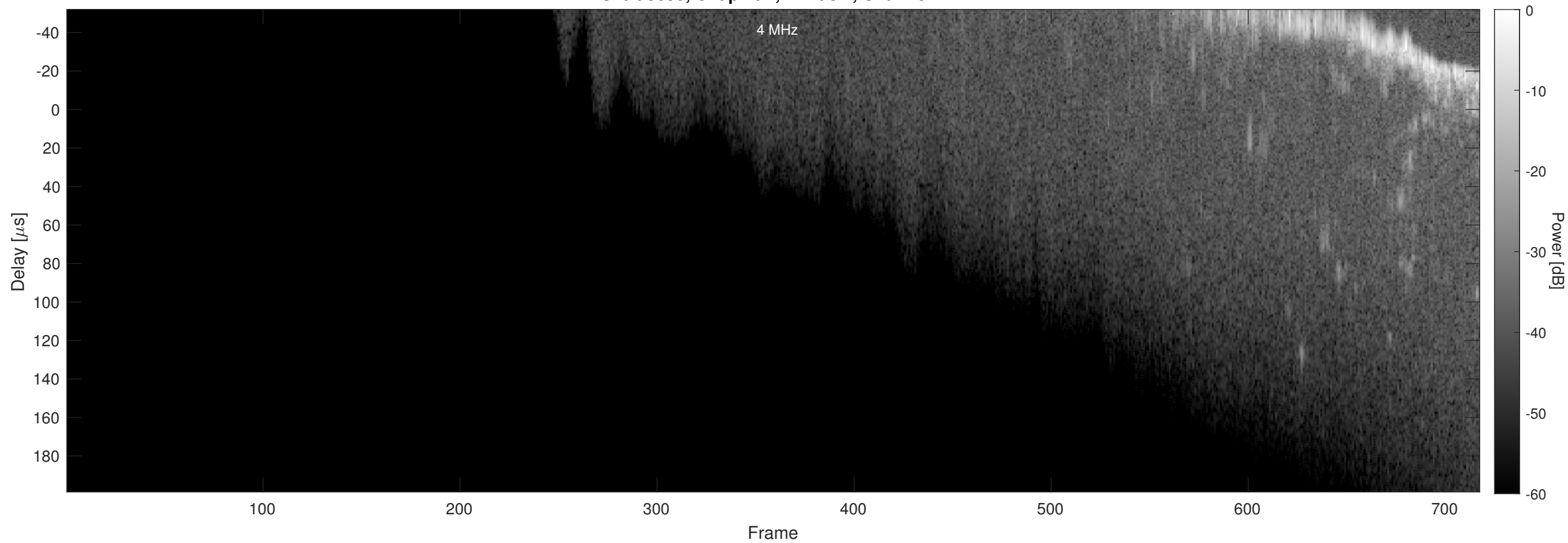
Orbit 3095, Chapman, Window, Channel 2
