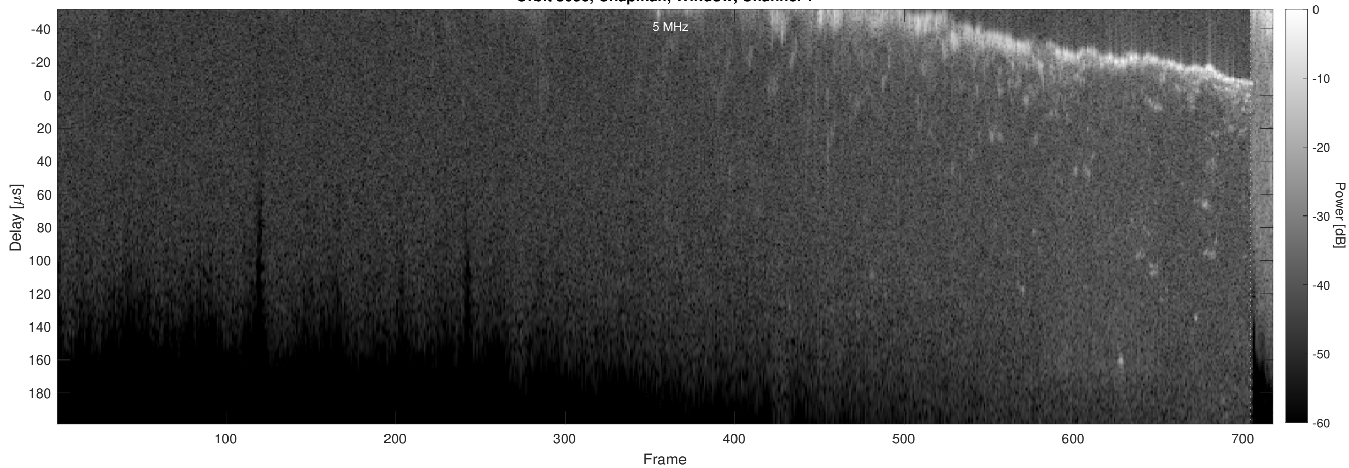
Orbit 3095, Chapman, Window, Channel 2
