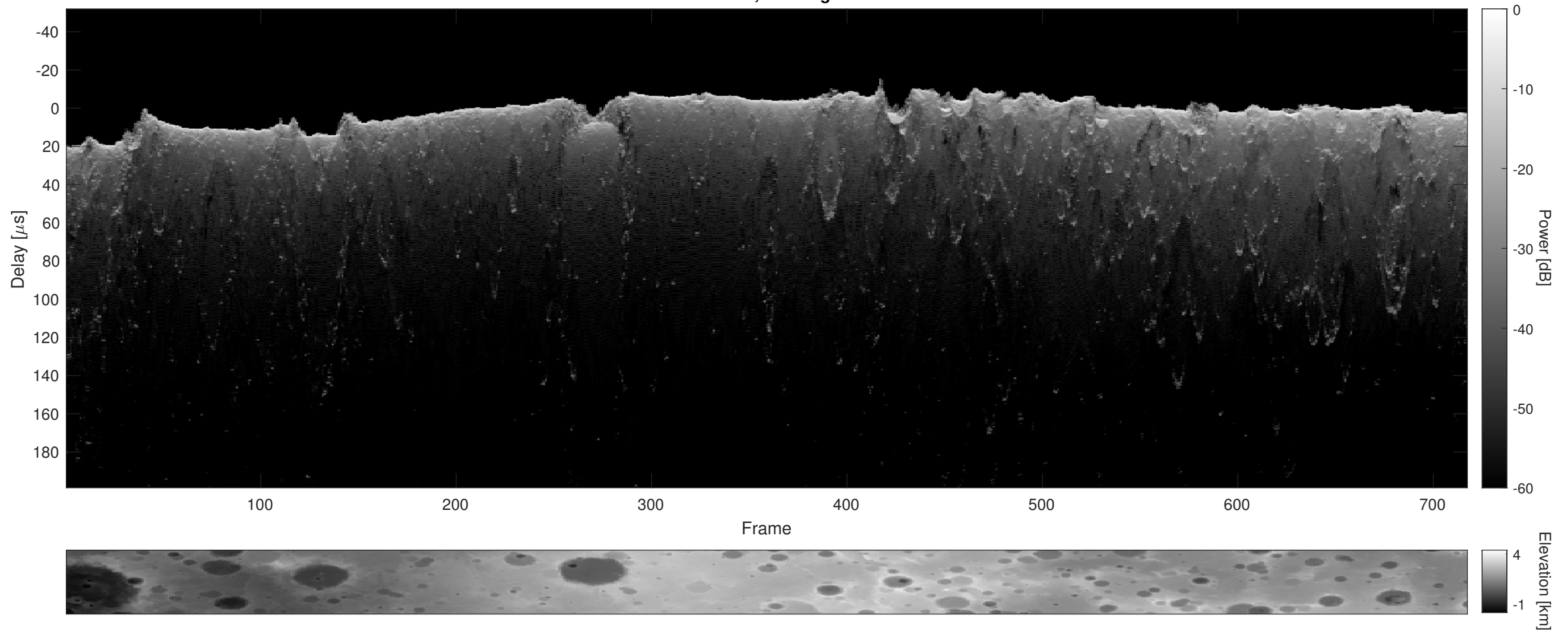
Orbit 3095, Cluttergram
