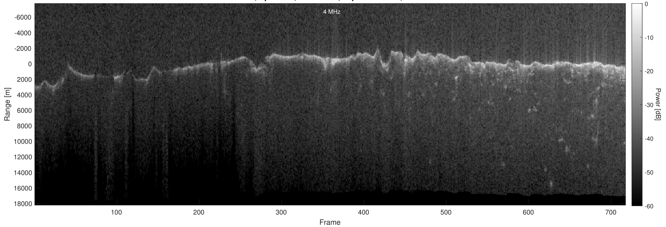
Orbit 3095, Optimized, No Window, Depth-Corrected, Channel 2
