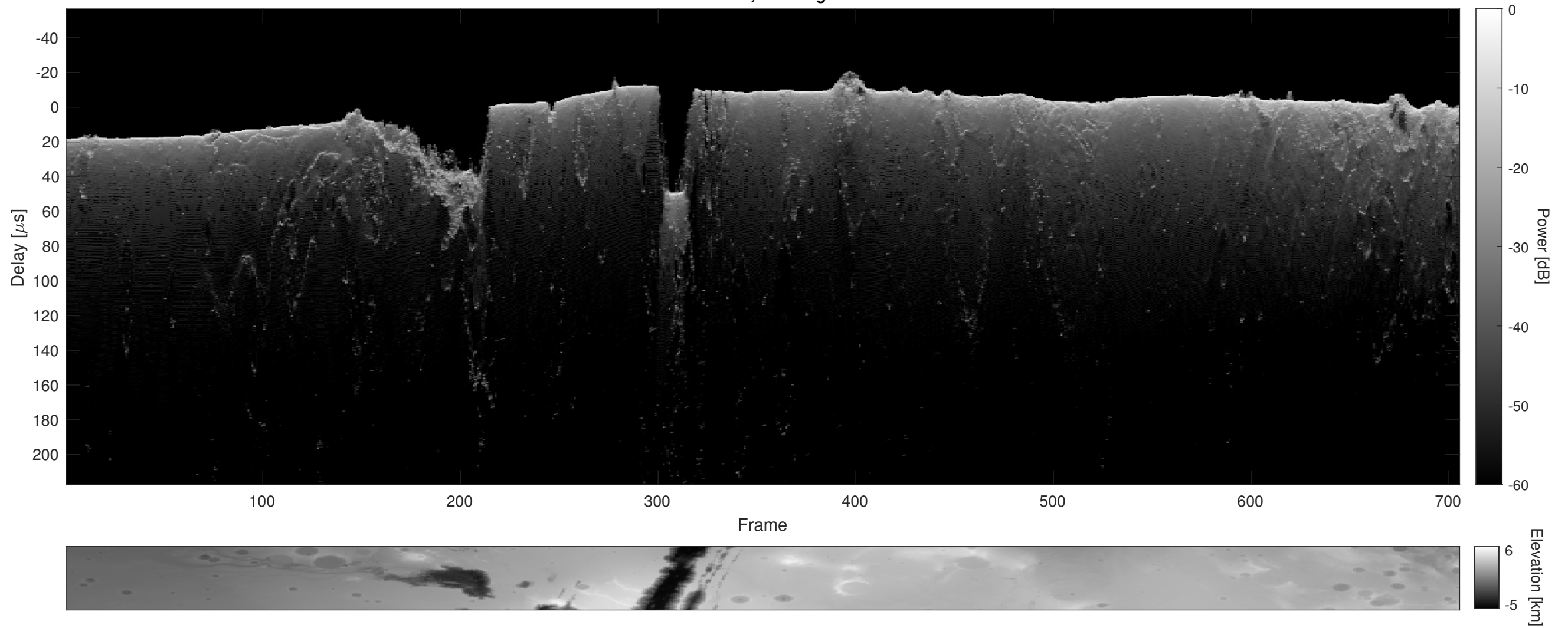
Orbit 3096, Cluttergram
