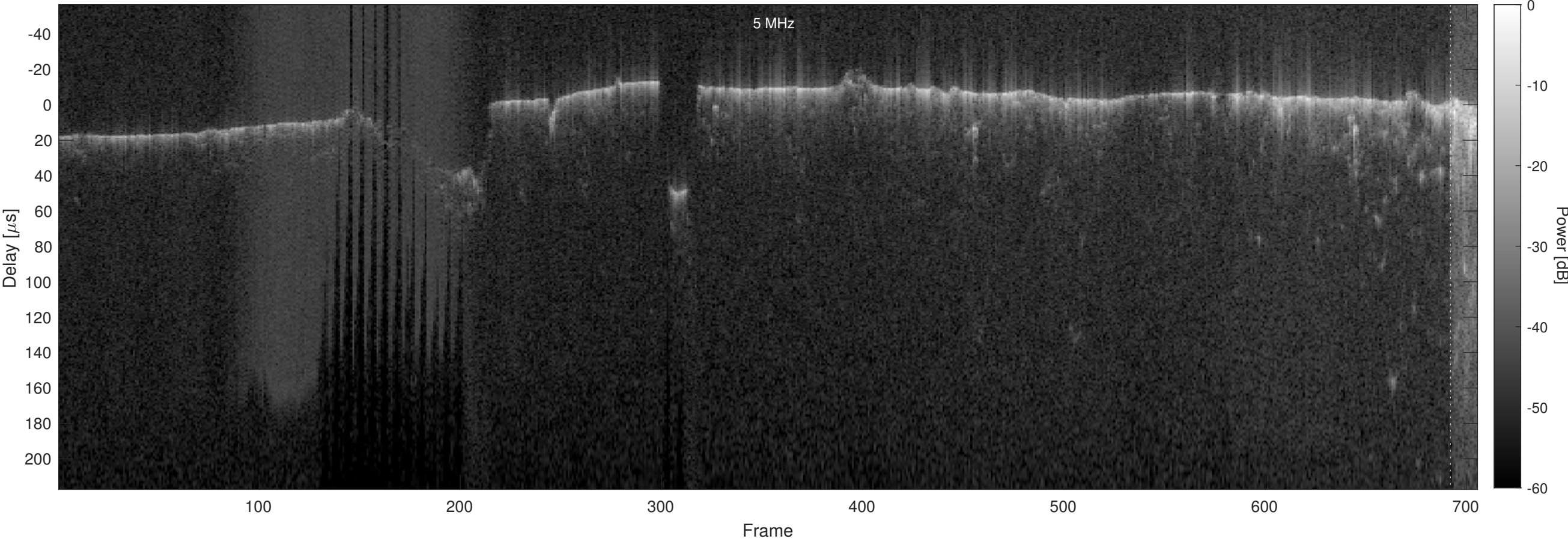
Orbit 3096, Optimized, No Window, Channel 2
