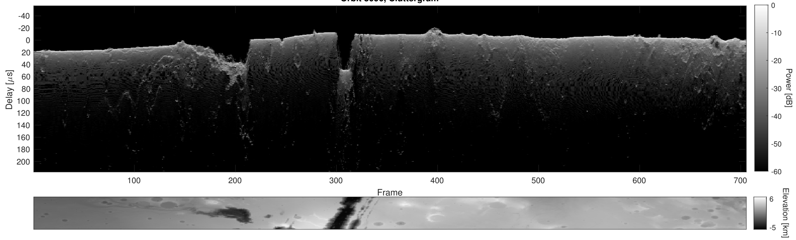
Orbit 3096, Cluttergram
