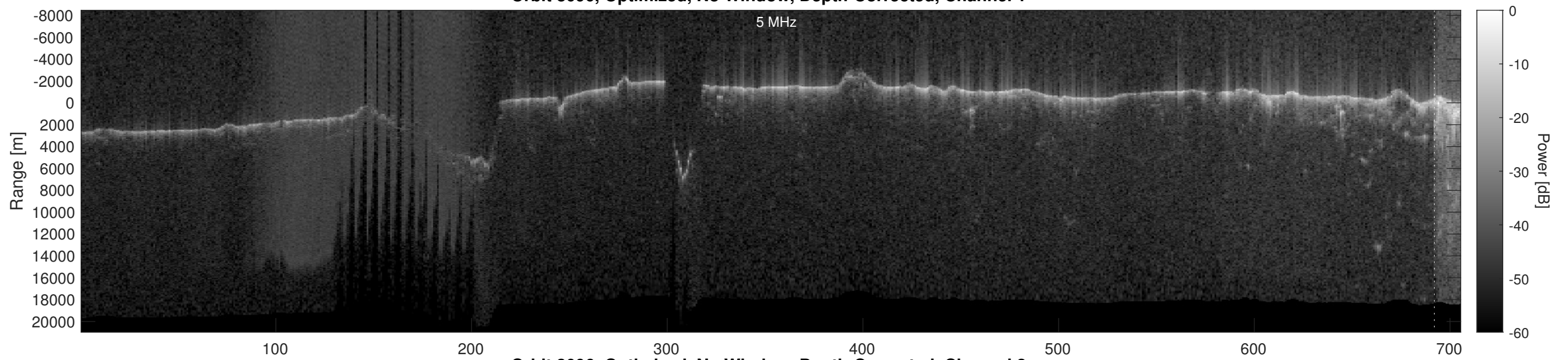
Orbit 3096, Optimized, No Window, Depth-Corrected, Channel 2
