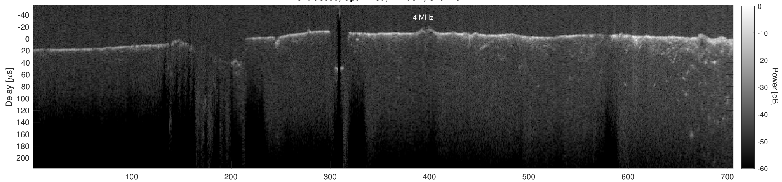
Orbit 3096, Cluttergram
