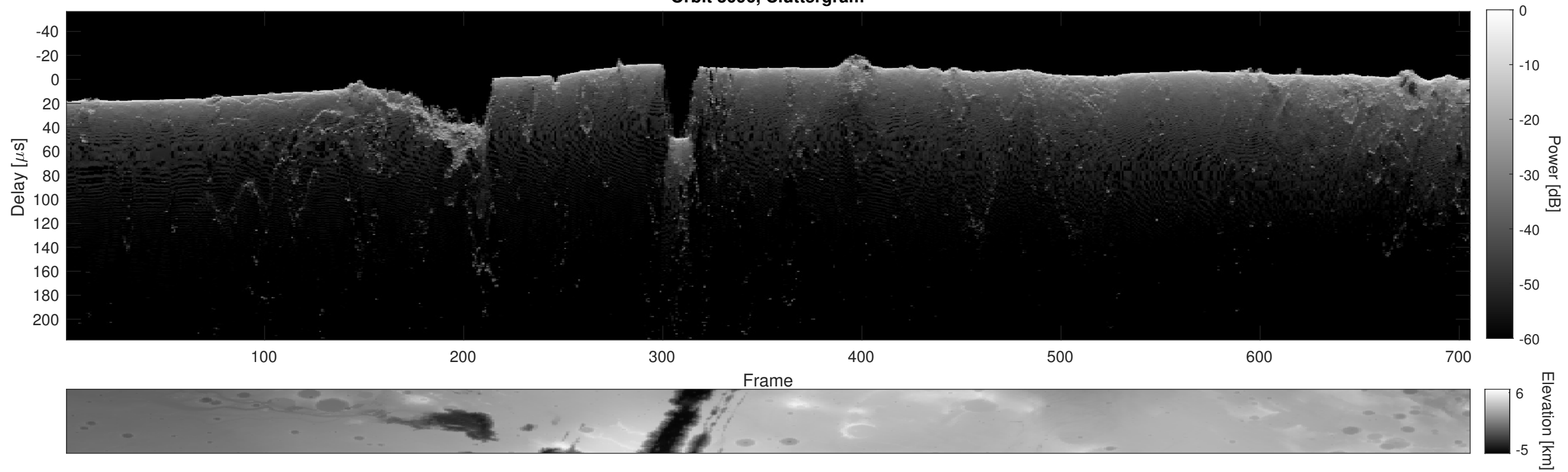
Orbit 3096, Cluttergram
