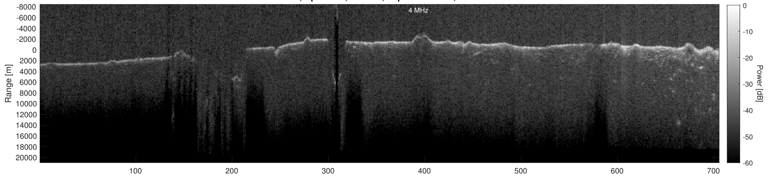
Orbit 3096, Depth-Corrected Cluttergram
