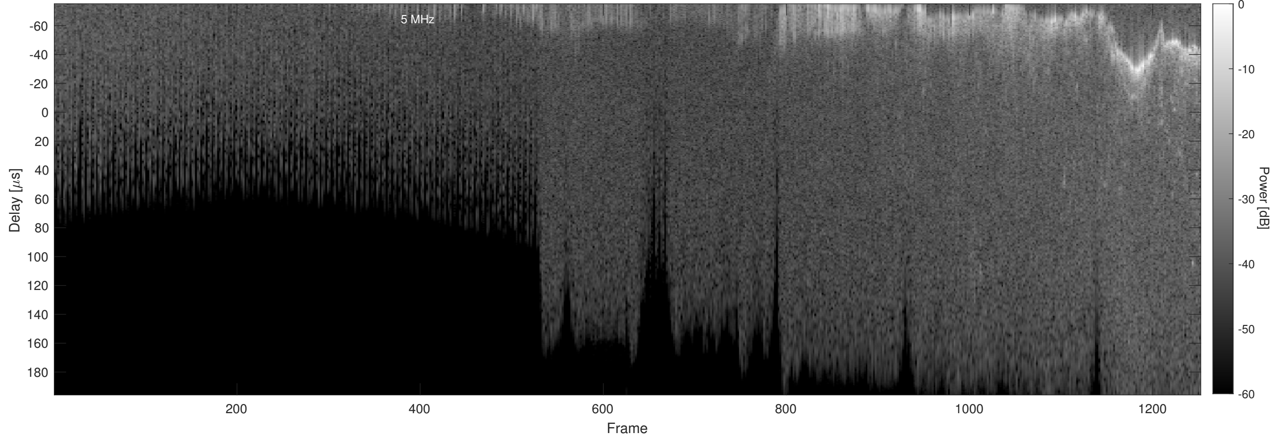
Orbit 3097, Chapman, No Window, Channel 2
