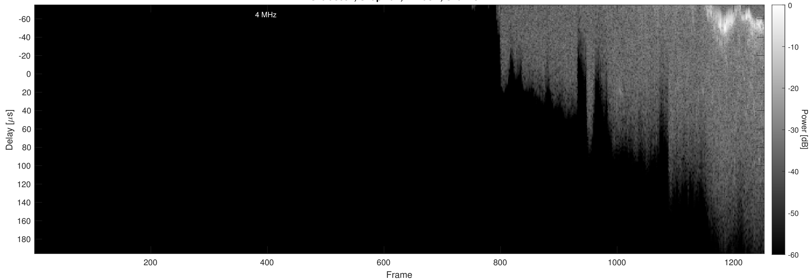
Orbit 3097, Chapman, Window, Channel 2
