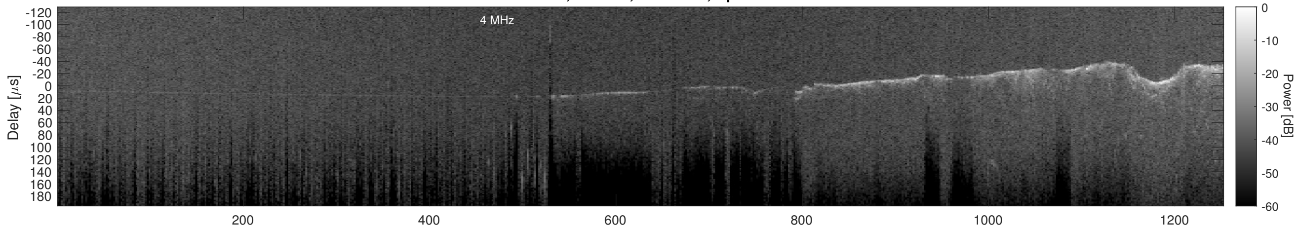
Orbit 3097, Cluttergram
