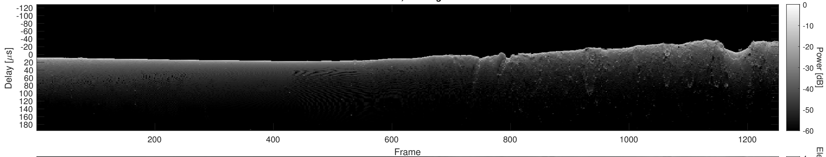
Orbit 3097, Cluttergram
