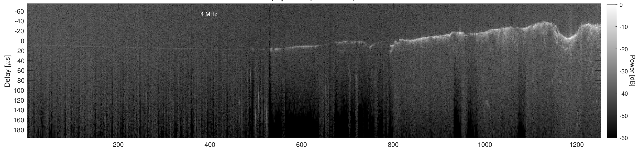
Orbit 3097, Cluttergram
