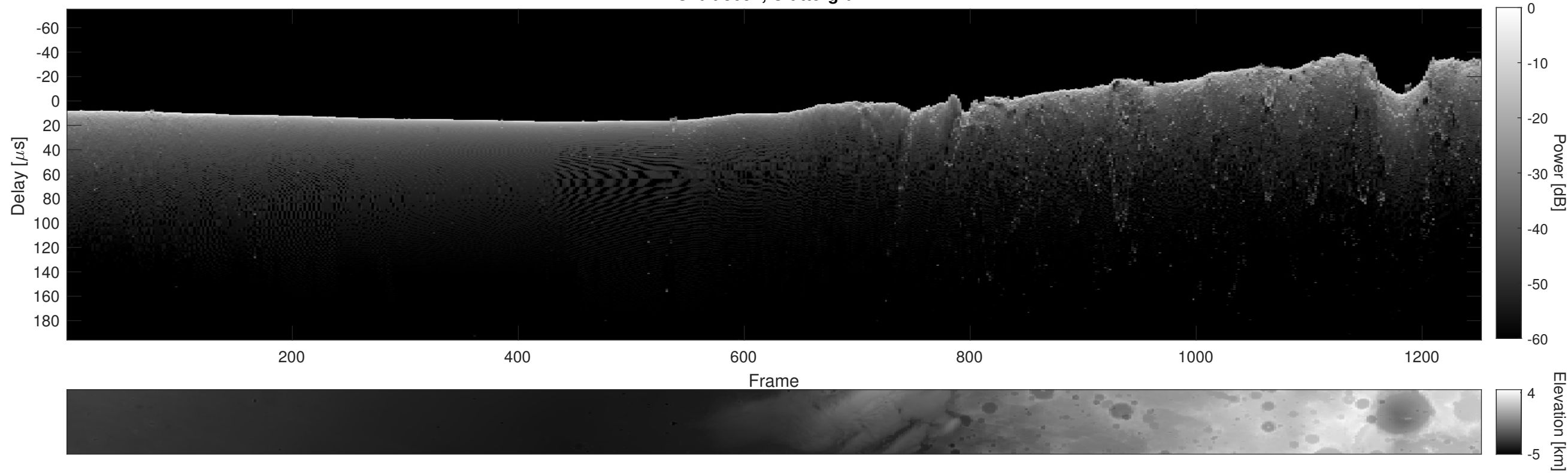
Orbit 3097, Cluttergram
