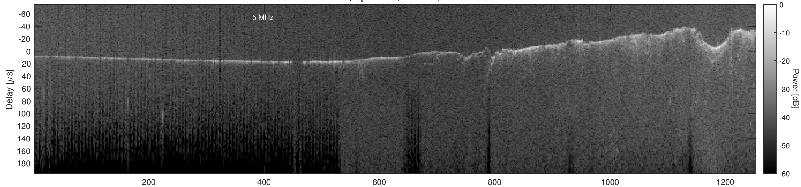
Orbit 3097, Optimized, Window, Channel 2
