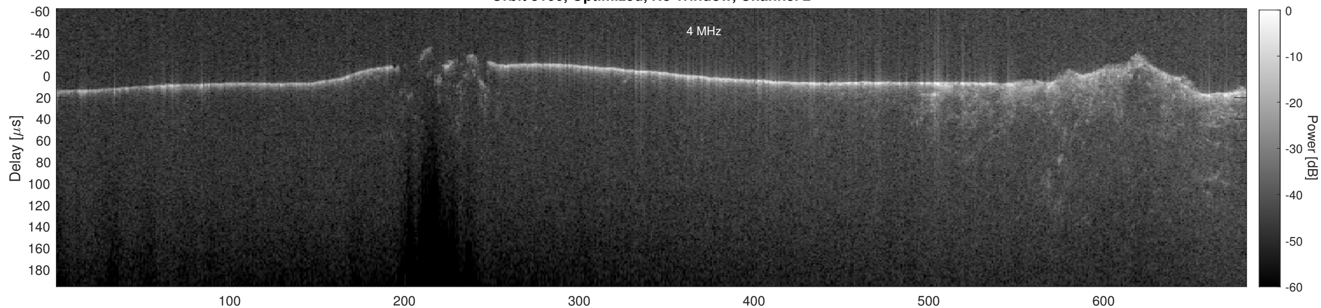
Orbit 3100, Cluttergram
