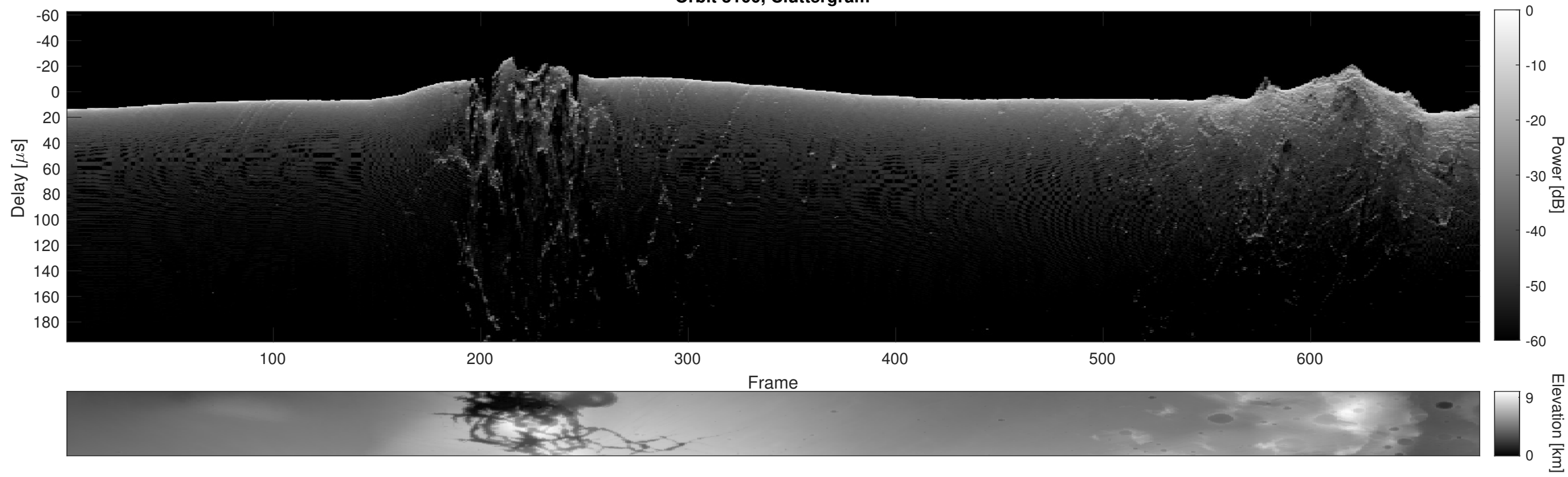
Orbit 3100, Cluttergram
