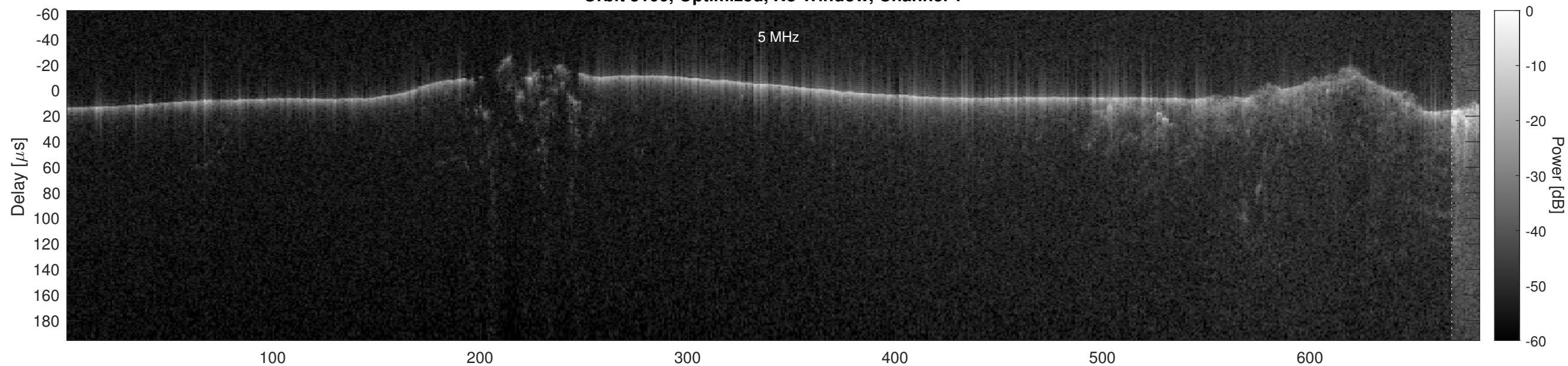
Orbit 3100, Optimized, No Window, Channel 2
