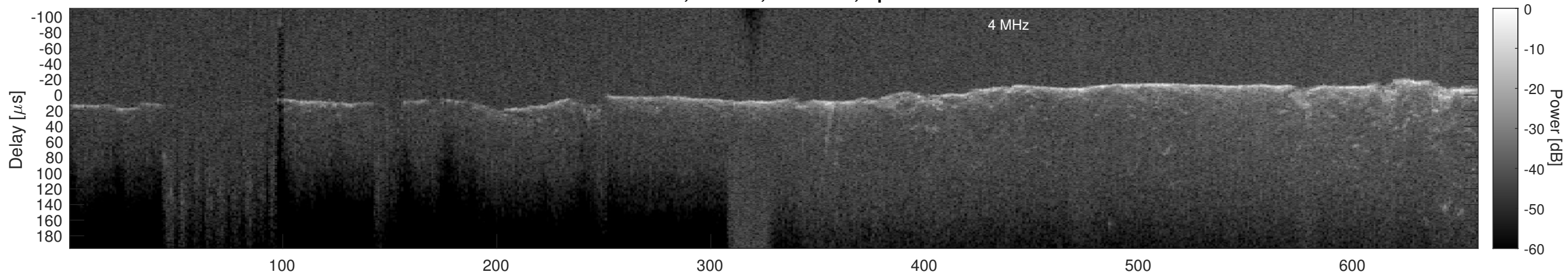
Orbit 3103, Cluttergram
