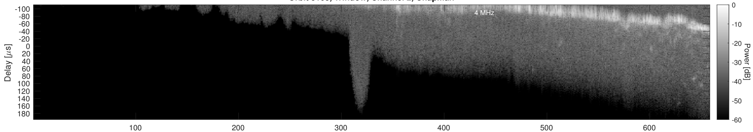
Orbit 3103, Window, Channel 2, Optimized
