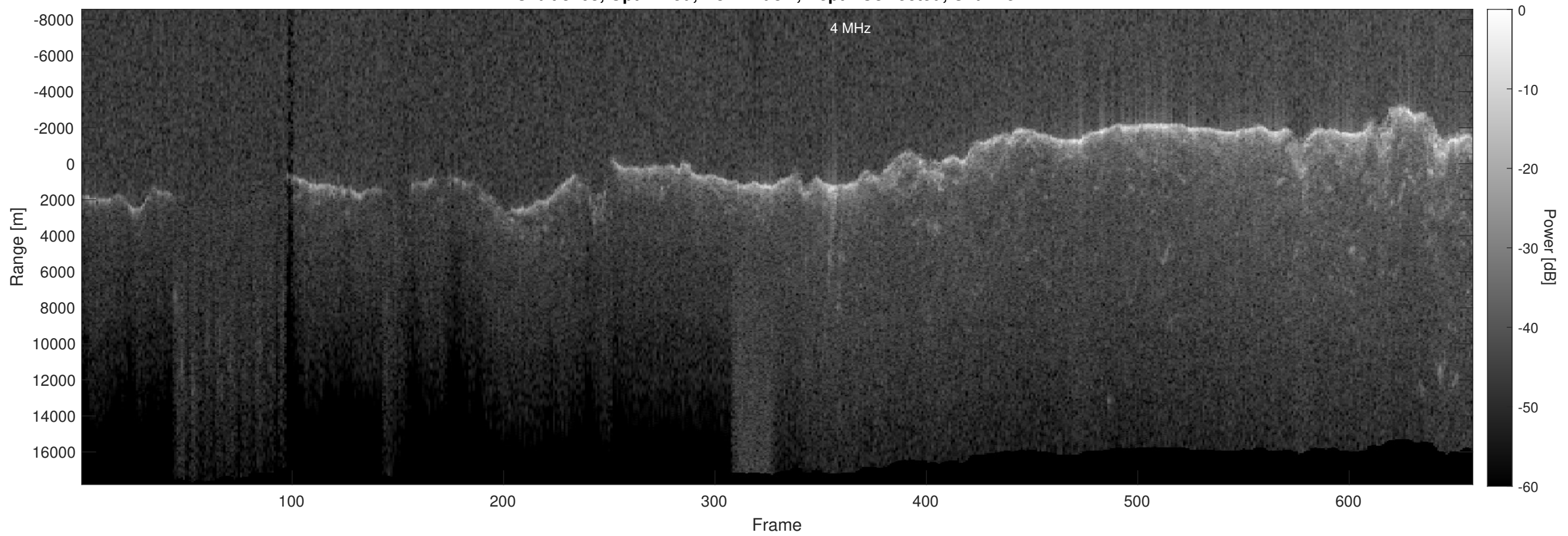
Orbit 3103, Optimized, No Window, Depth-Corrected, Channel 2
