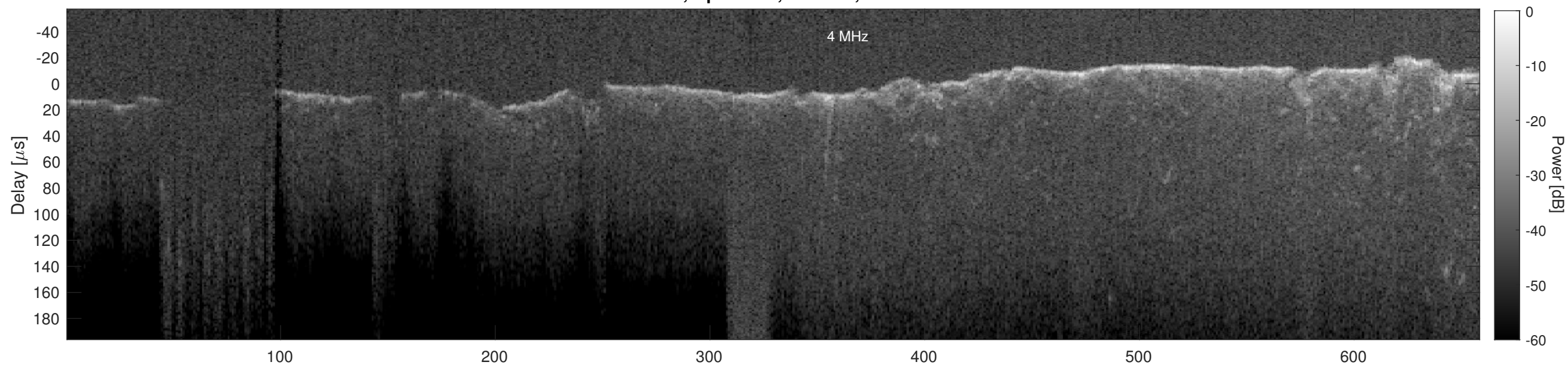
Orbit 3103, Cluttergram
