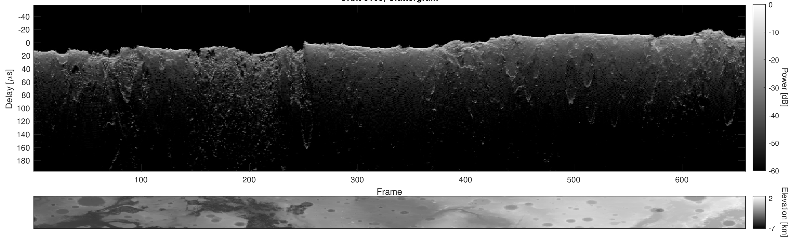
Orbit 3103, Cluttergram
