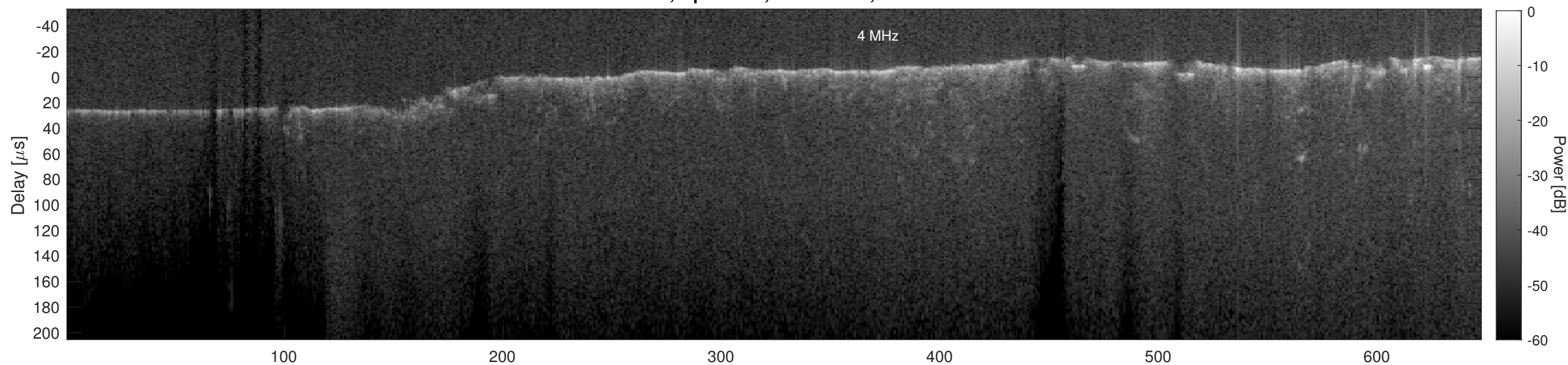
Orbit 3105, Cluttergram
