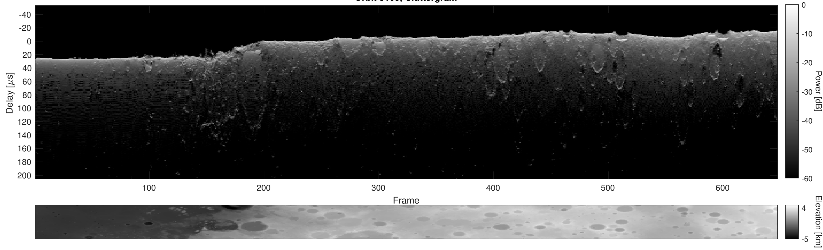
Orbit 3105, Cluttergram
