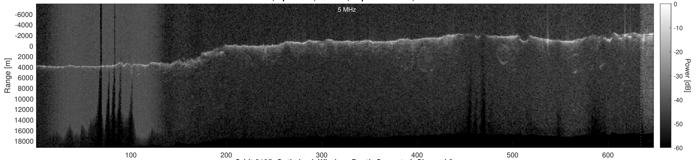
Orbit 3105, Optimized, Window, Depth-Corrected, Channel 2
