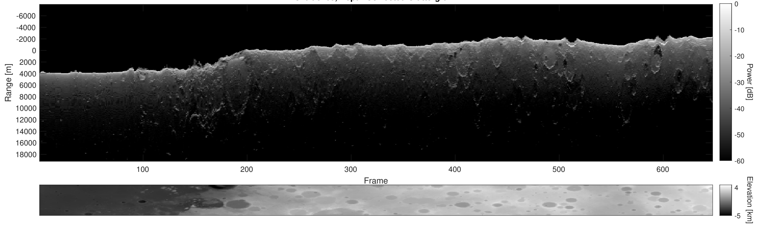
Orbit 3105, Depth-Corrected Cluttergram
