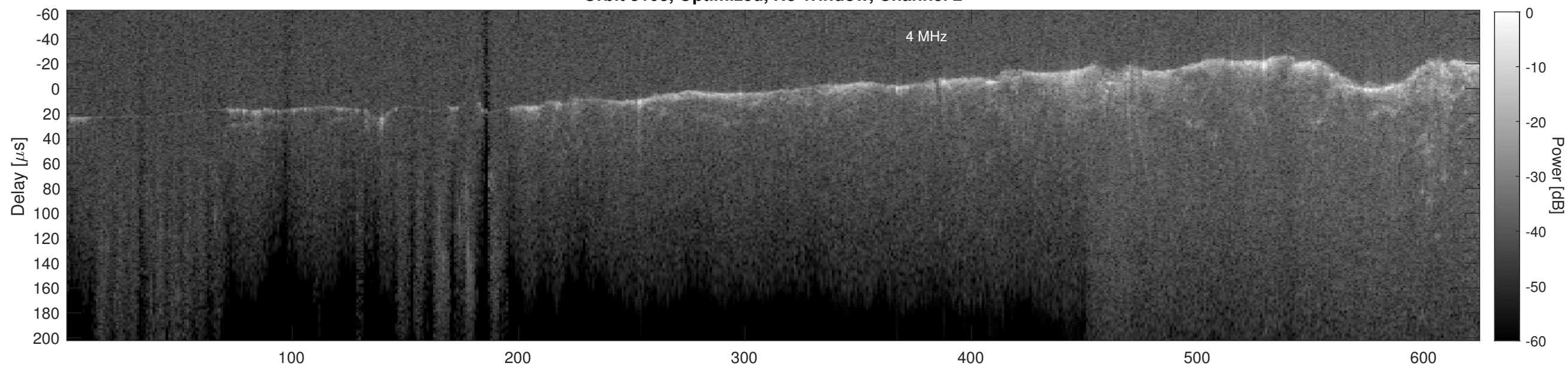
Orbit 3108, Cluttergram
