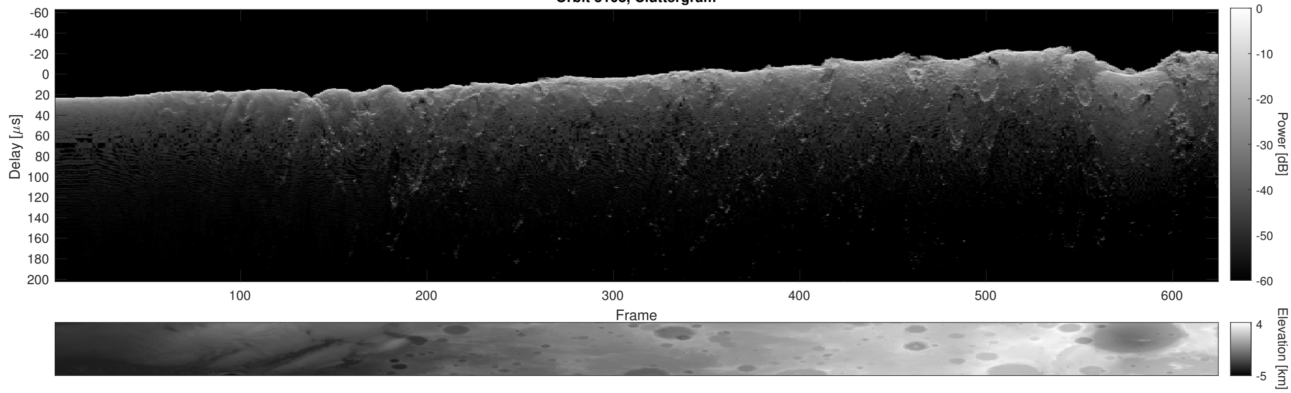
Orbit 3108, Cluttergram
