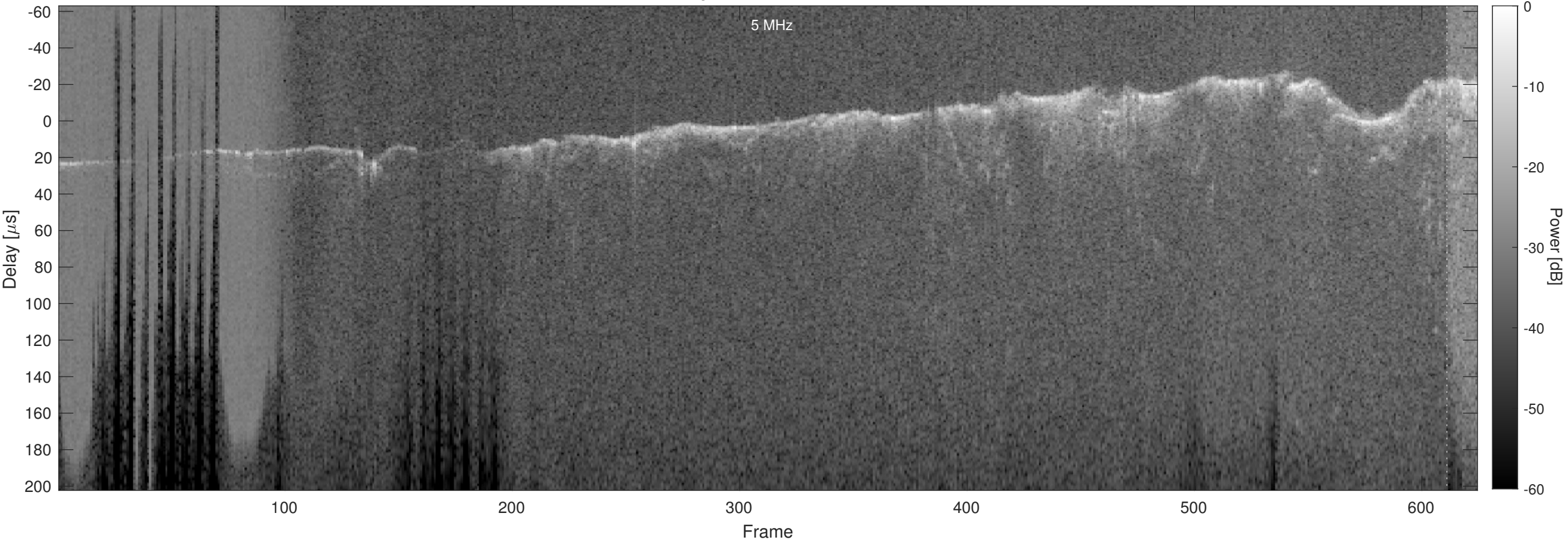
Orbit 3108, Optimized, Window, Channel 2
