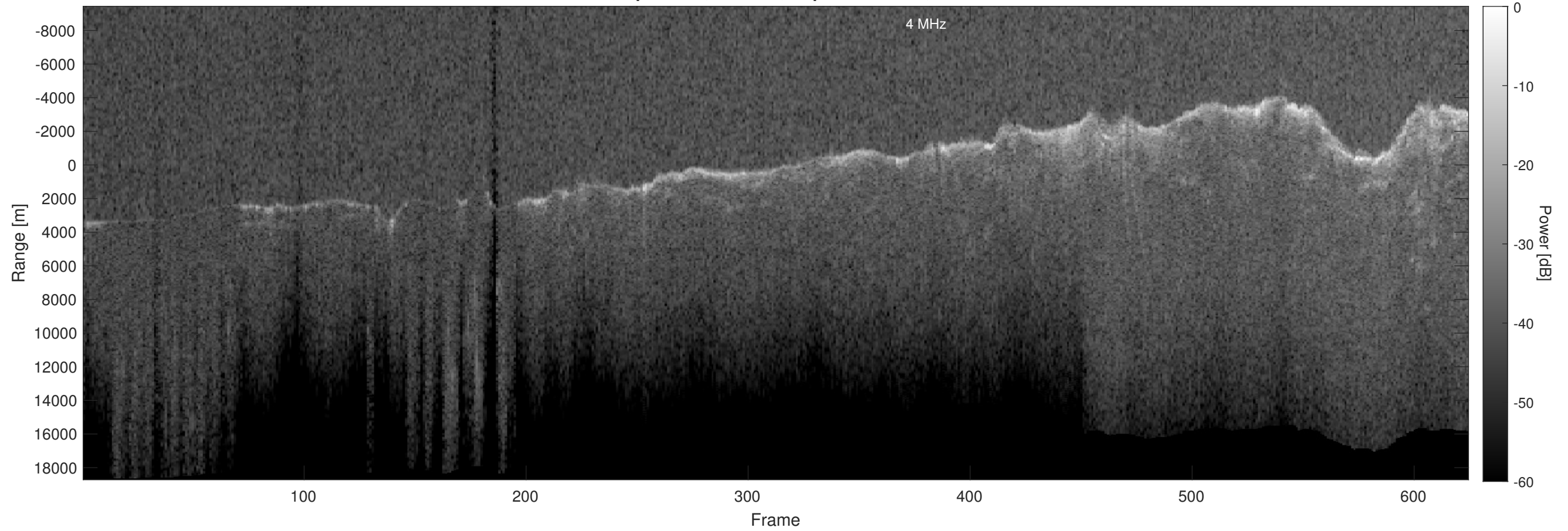
Orbit 3108, Optimized, Window, Depth-Corrected, Channel 2
