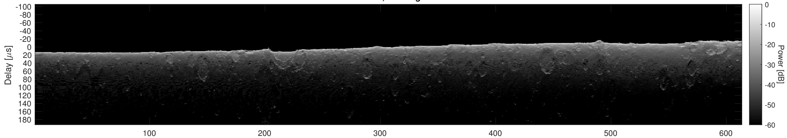
Orbit 3110, Cluttergram
