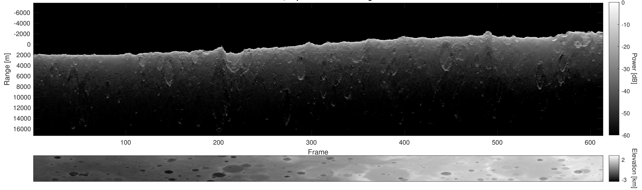
Orbit 3110, Depth-Corrected Cluttergram
