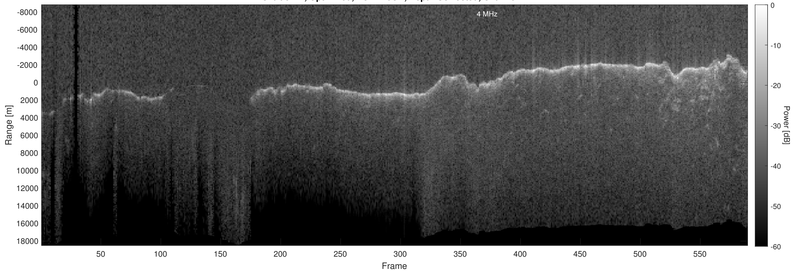
Orbit 3114, Optimized, No Window, Depth-Corrected, Channel 2
