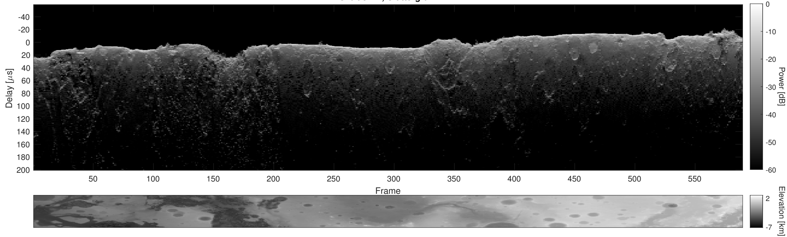
Orbit 3114, Cluttergram
