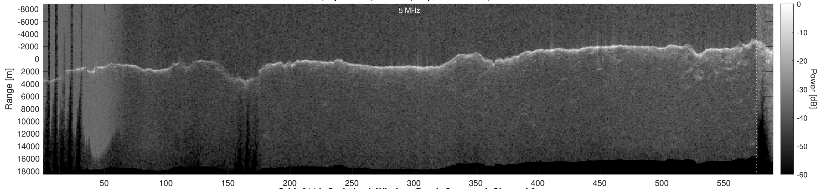
Orbit 3114, Optimized, Window, Depth-Corrected, Channel 2
