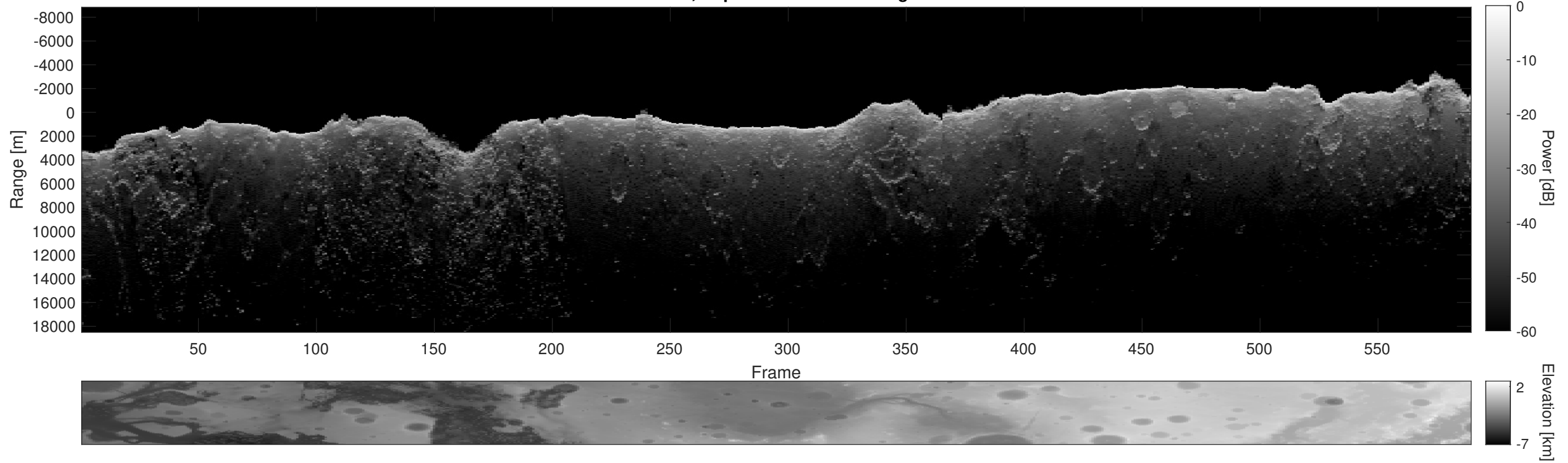
Orbit 3114, Depth-Corrected Cluttergram
