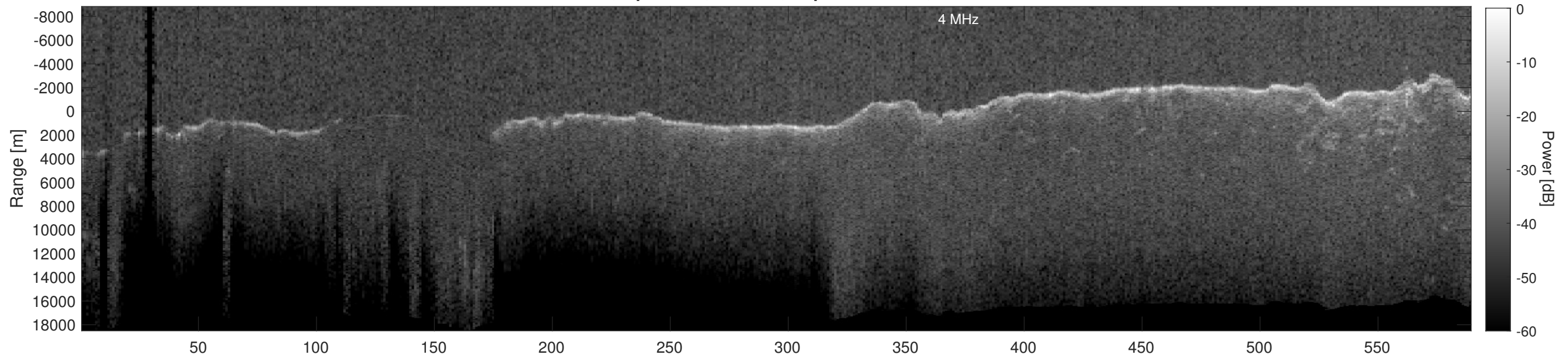
Orbit 3114, Depth-Corrected Cluttergram
