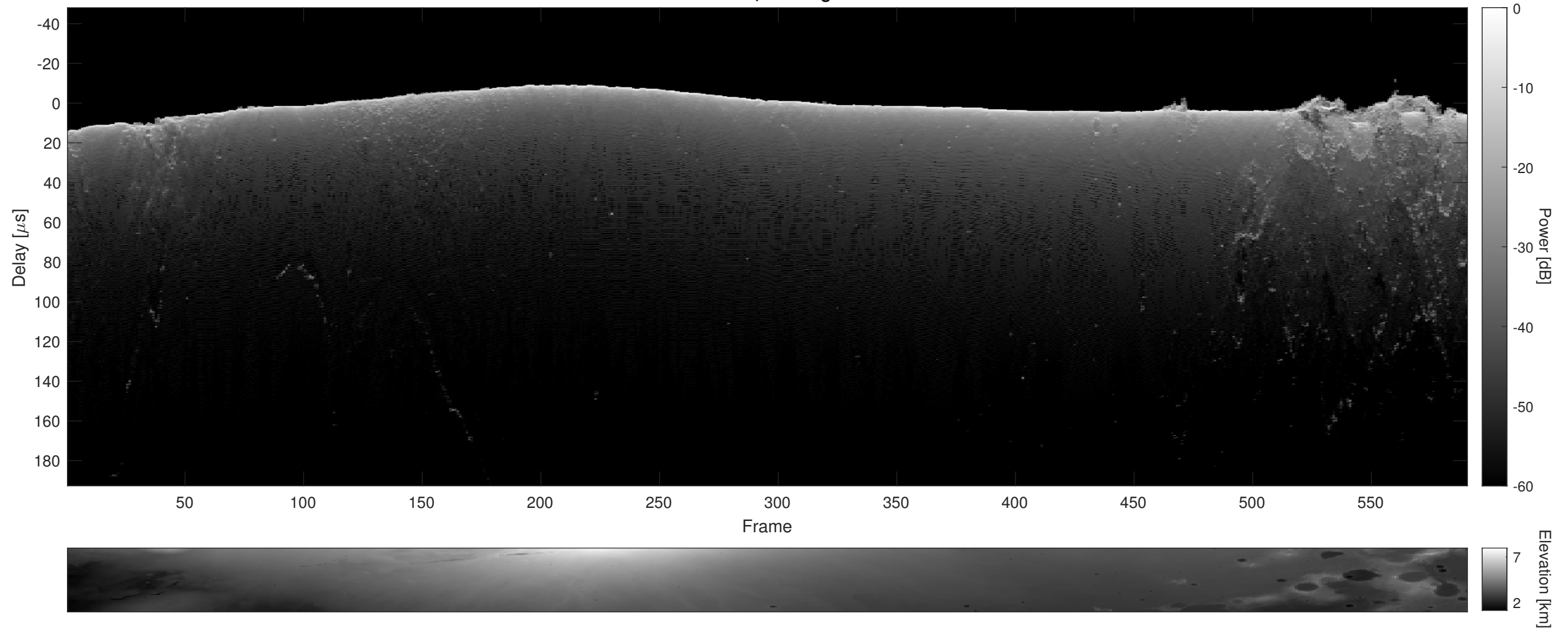
Orbit 3115, Cluttergram
