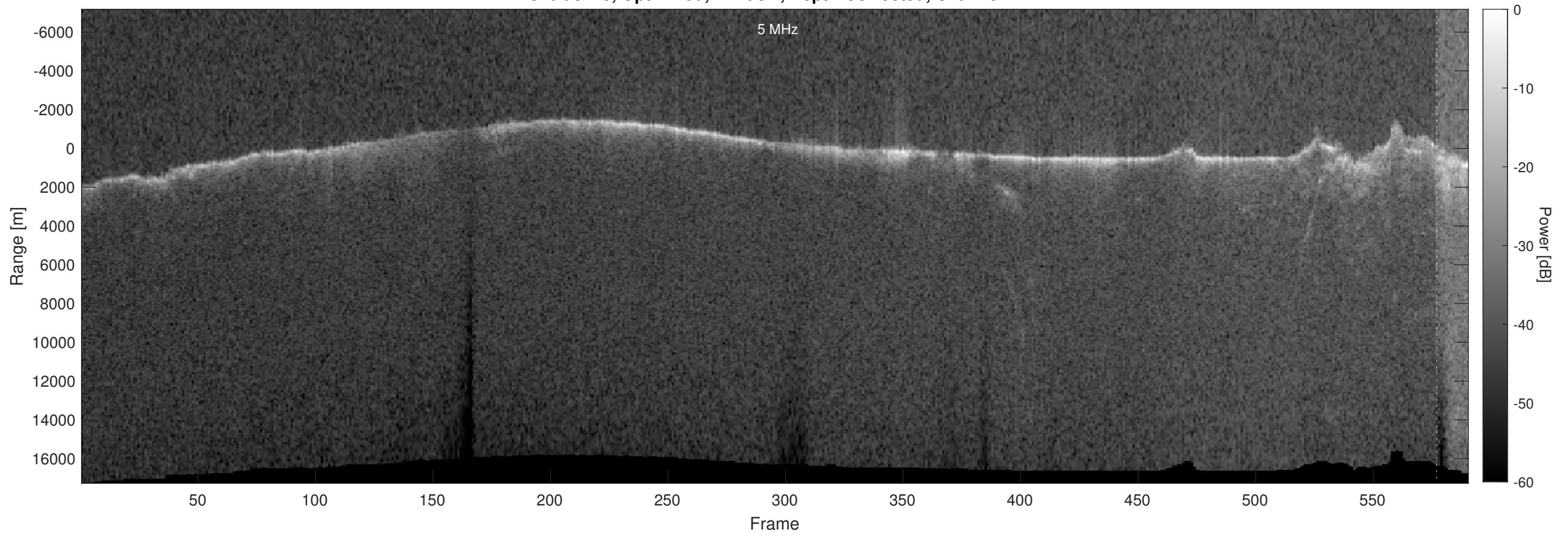
Orbit 3115, Optimized, Window, Depth-Corrected, Channel 2
