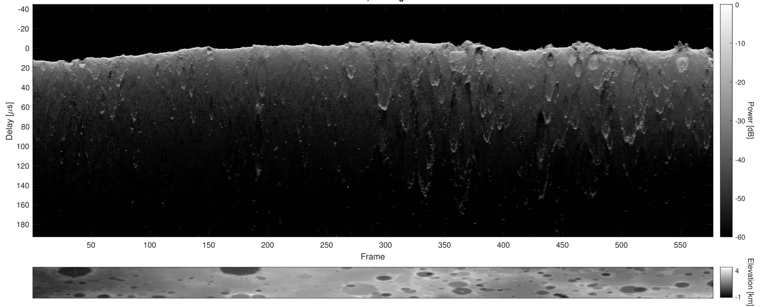
Orbit 3117, Cluttergram
