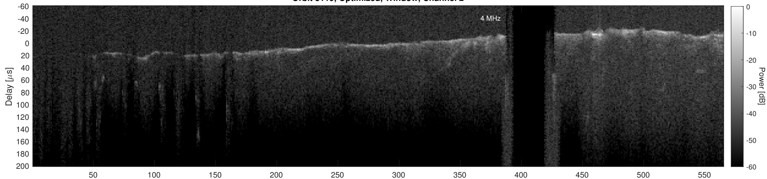
Orbit 3119, Cluttergram
