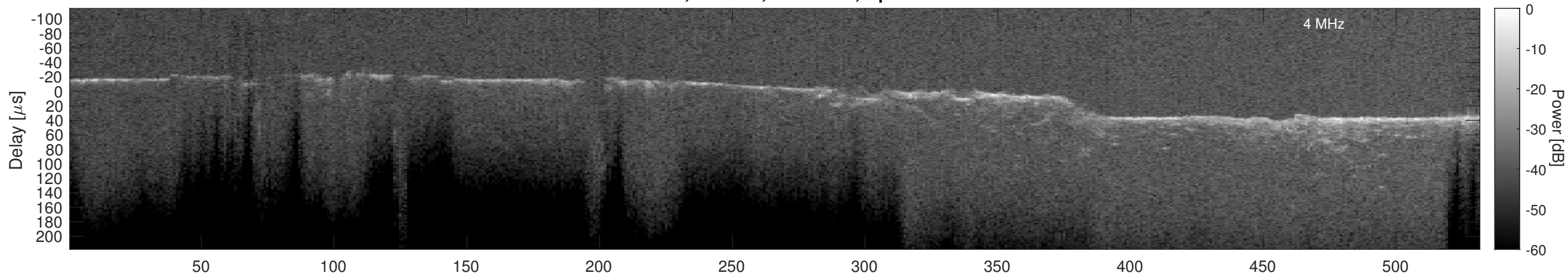
Orbit 3124, Cluttergram
