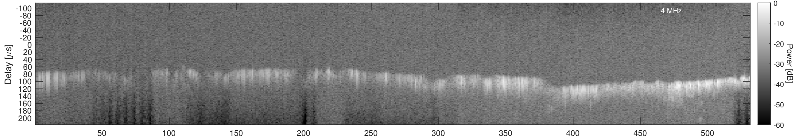
Orbit 3124, Window, Channel 2, Chapman
