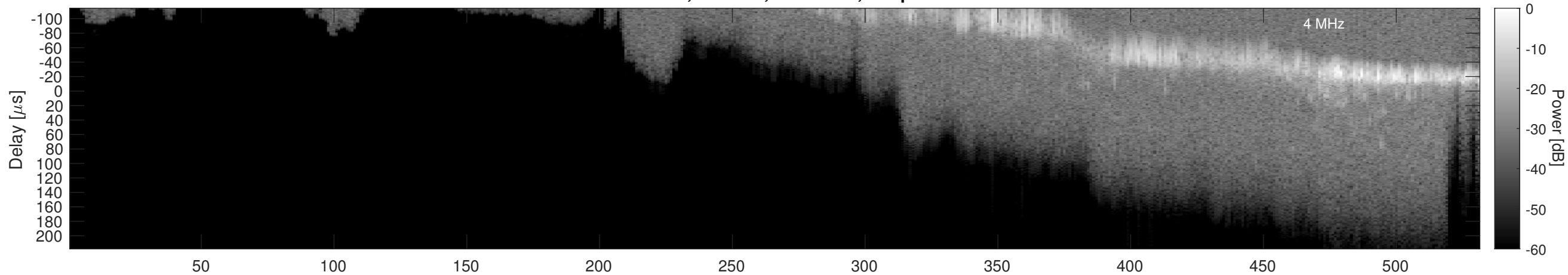
Orbit 3124, Window, Channel 2, Optimized
