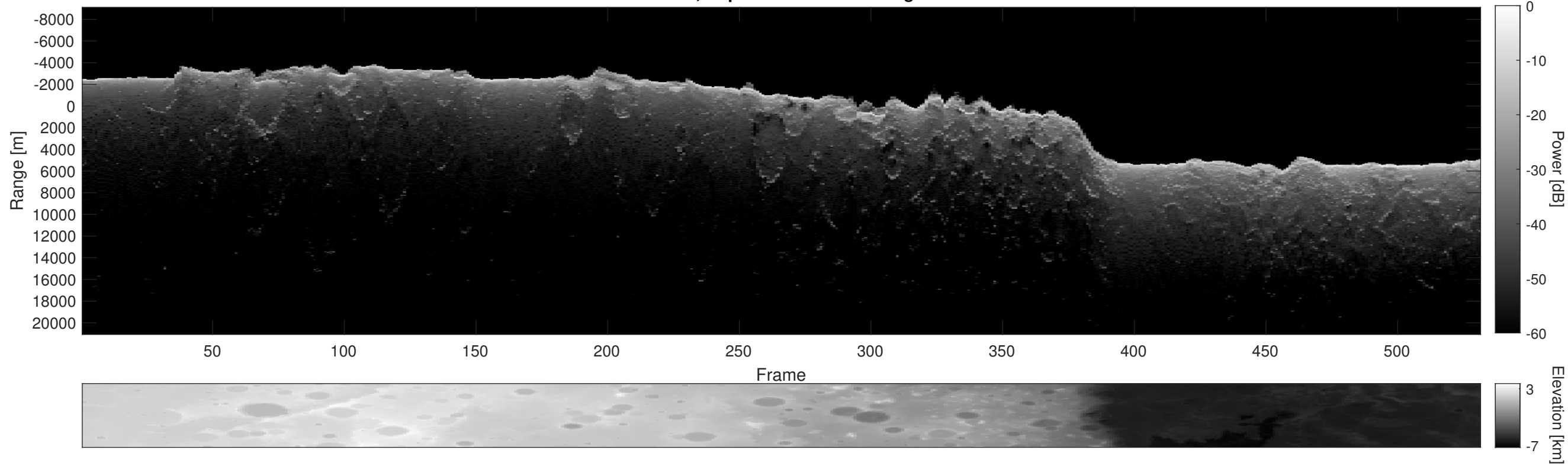
Orbit 3124, Depth-Corrected Cluttergram
