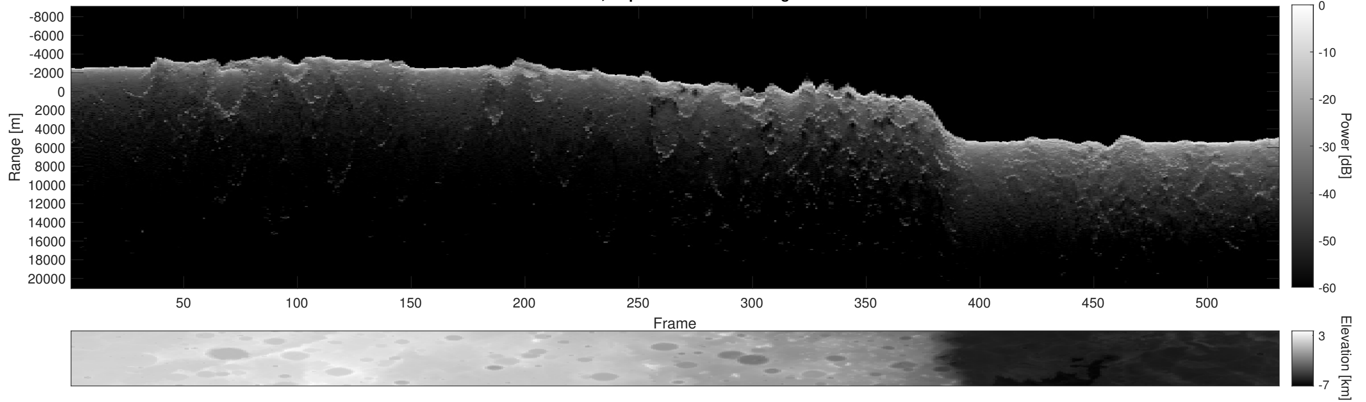
Orbit 3124, Depth-Corrected Cluttergram
