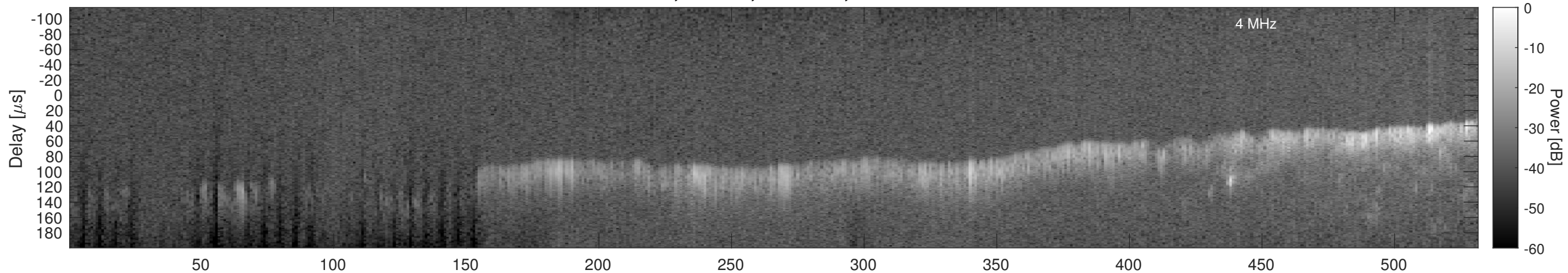
Orbit 3125, Window, Channel 2, Chapman
