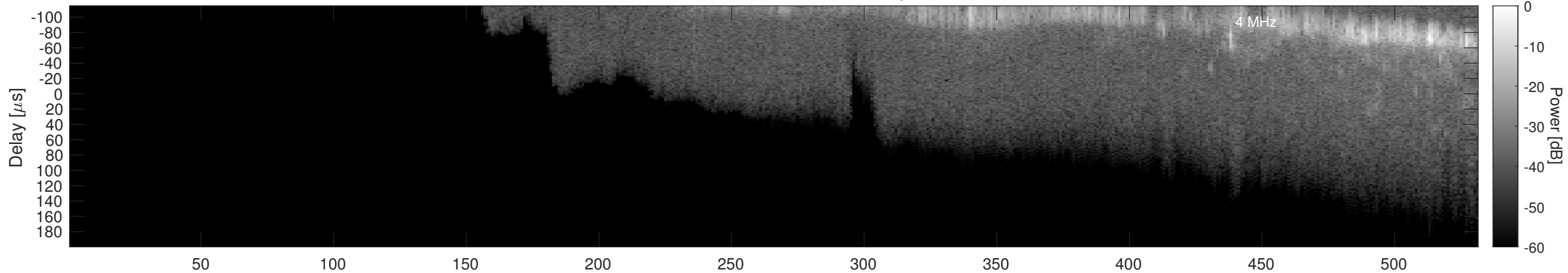
Orbit 3125, Window, Channel 2, Optimized
