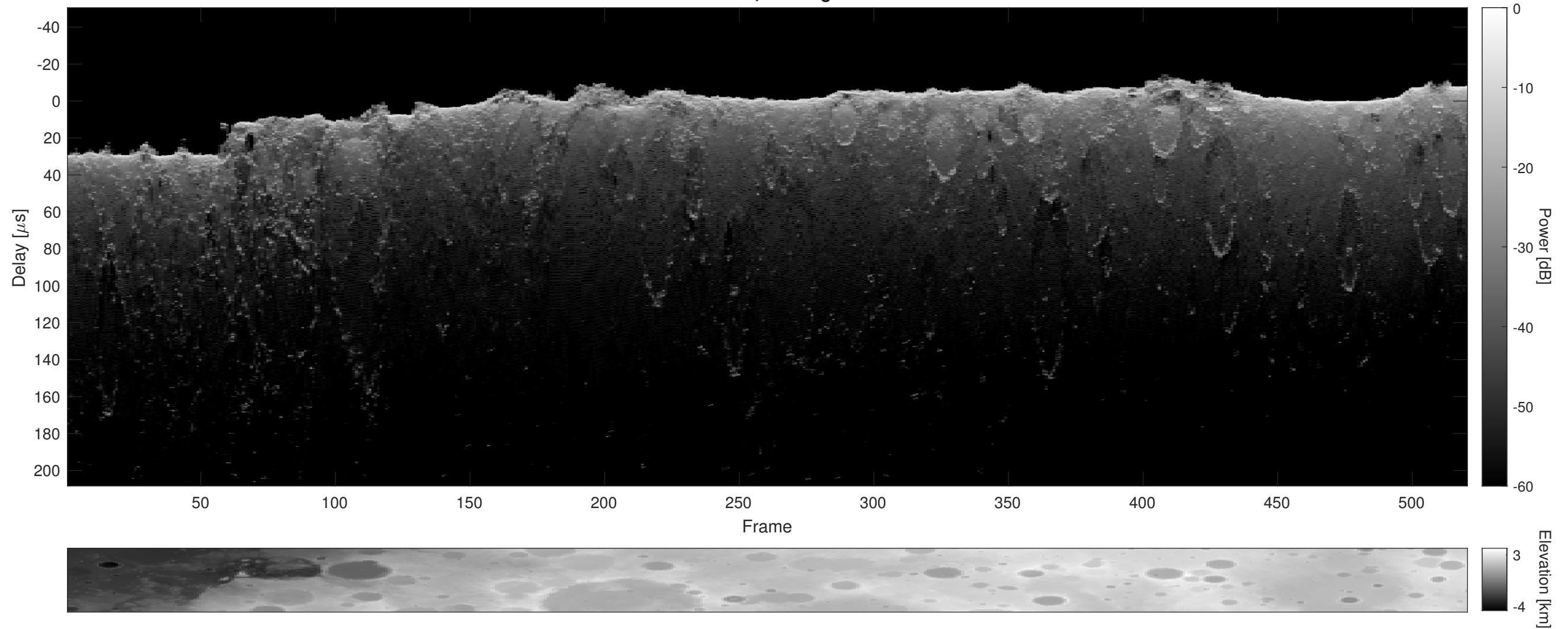
Orbit 3127, Cluttergram
