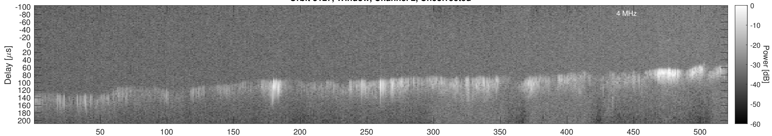
Orbit 3127, Window, Channel 2, Chapman
