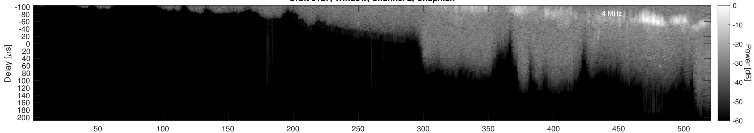
Orbit 3127, Window, Channel 2, Optimized
