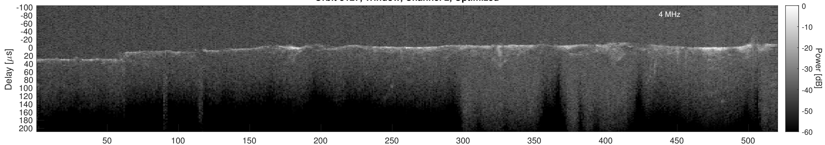
Orbit 3127, Cluttergram
