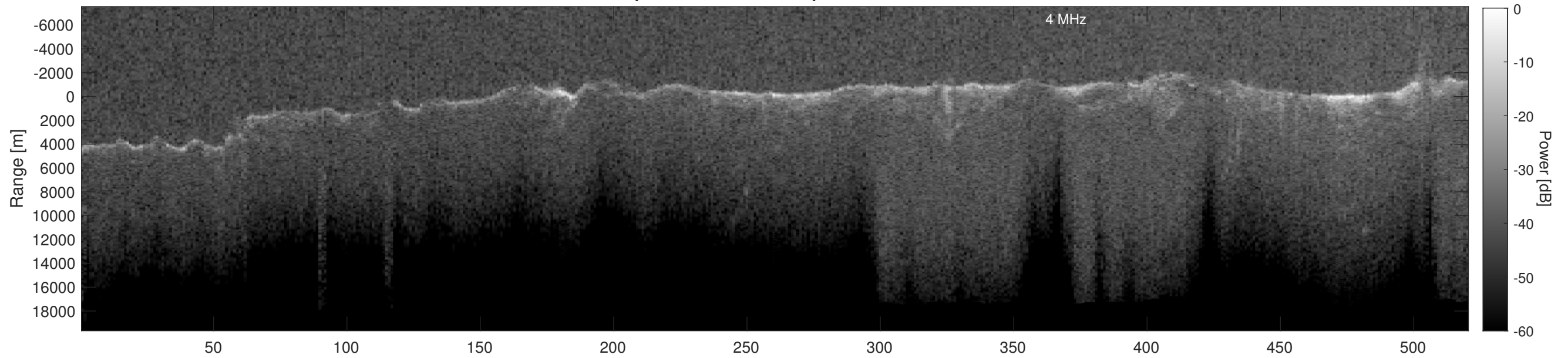
Orbit 3127, Depth-Corrected Cluttergram
