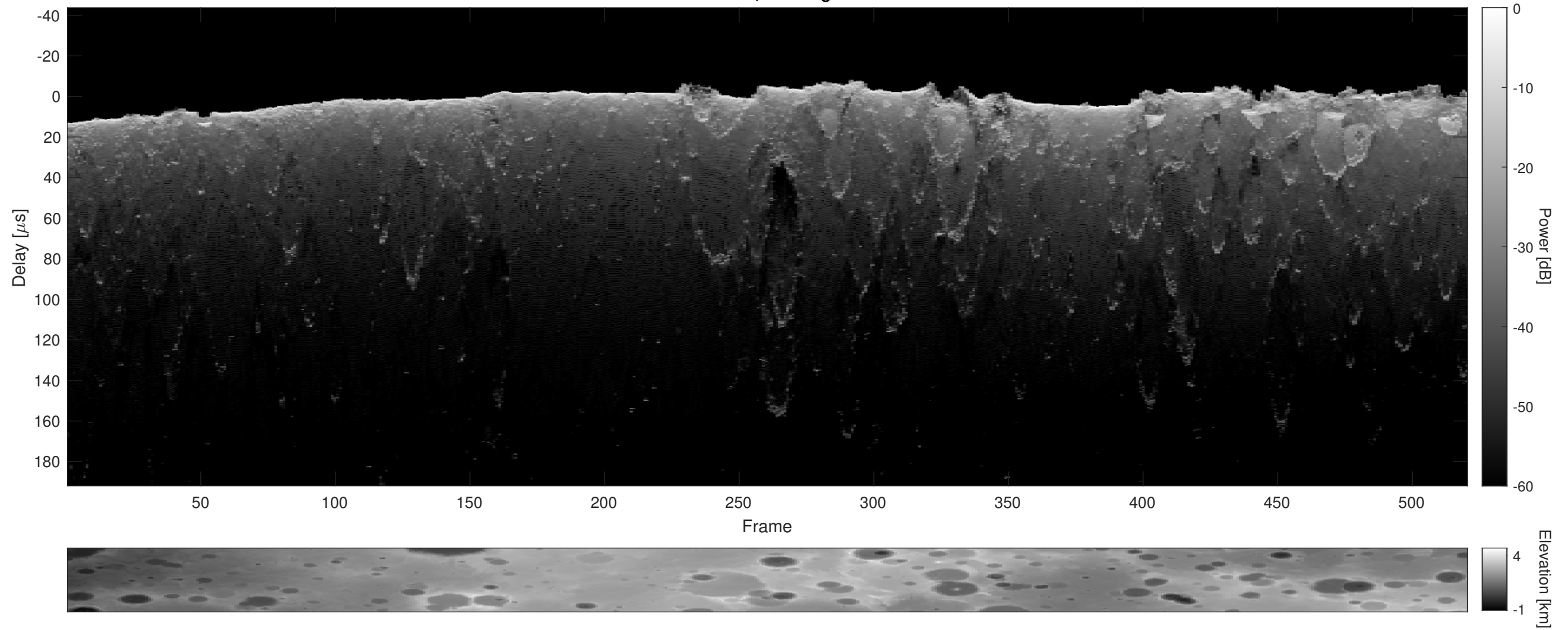
Orbit 3128, Cluttergram
