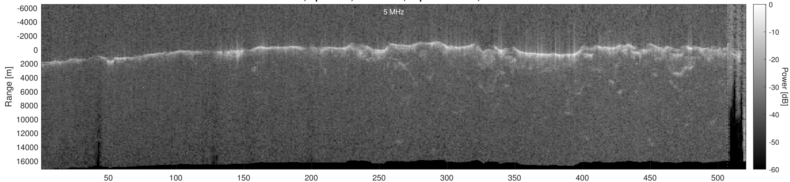
Orbit 3128, Optimized, No Window, Depth-Corrected, Channel 2
