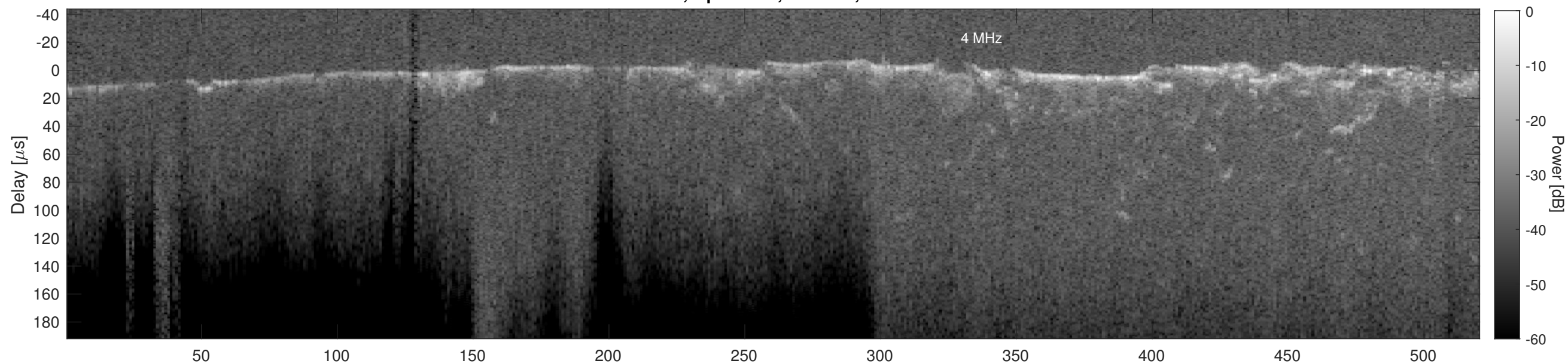
Orbit 3128, Cluttergram
