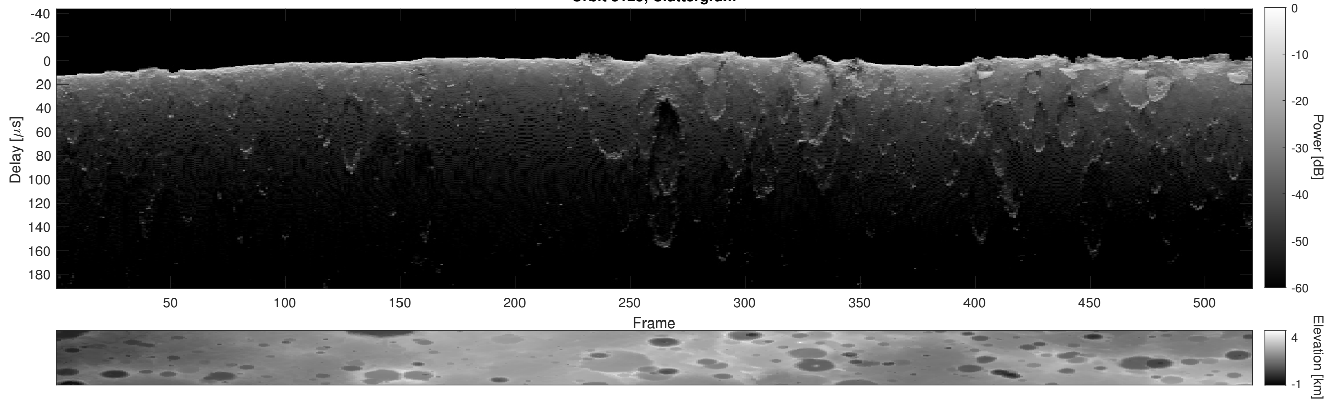
Orbit 3128, Cluttergram
