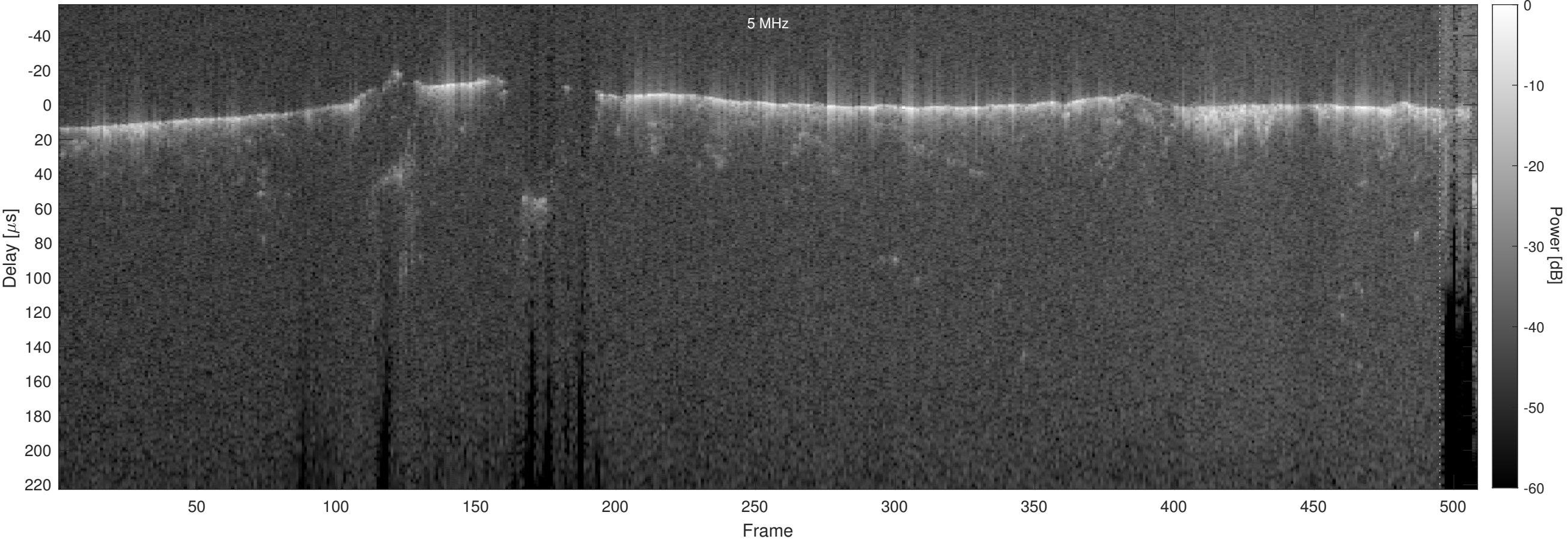
Orbit 3129, Optimized, No Window, Channel 2
