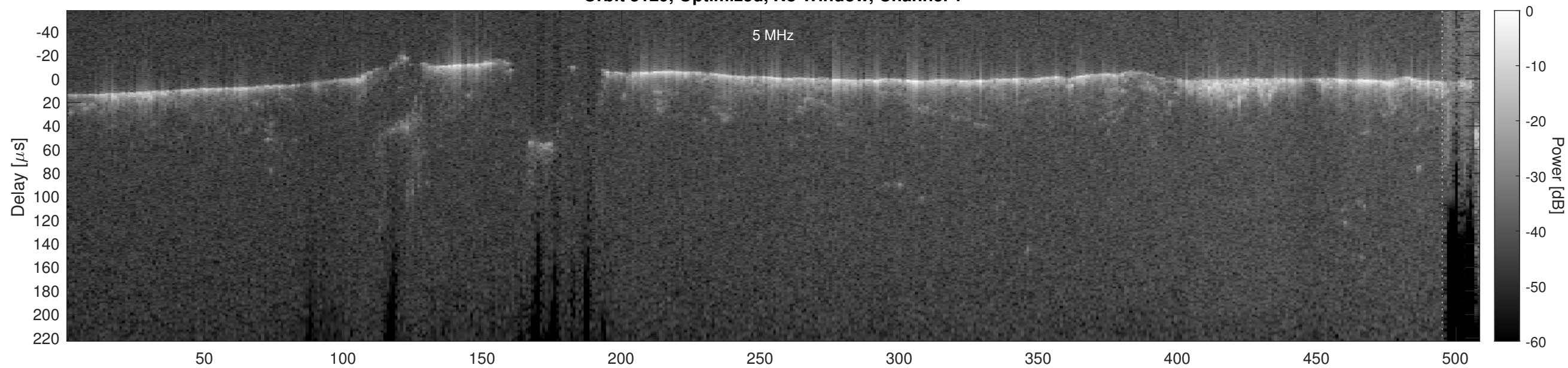
Orbit 3129, Optimized, No Window, Channel 2
