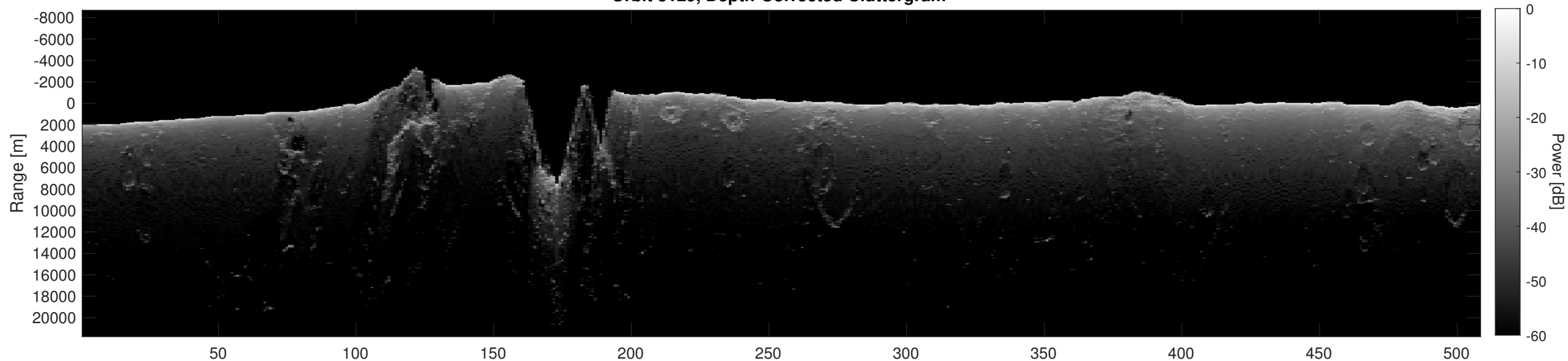
Orbit 3129, Depth-Corrected Cluttergram
