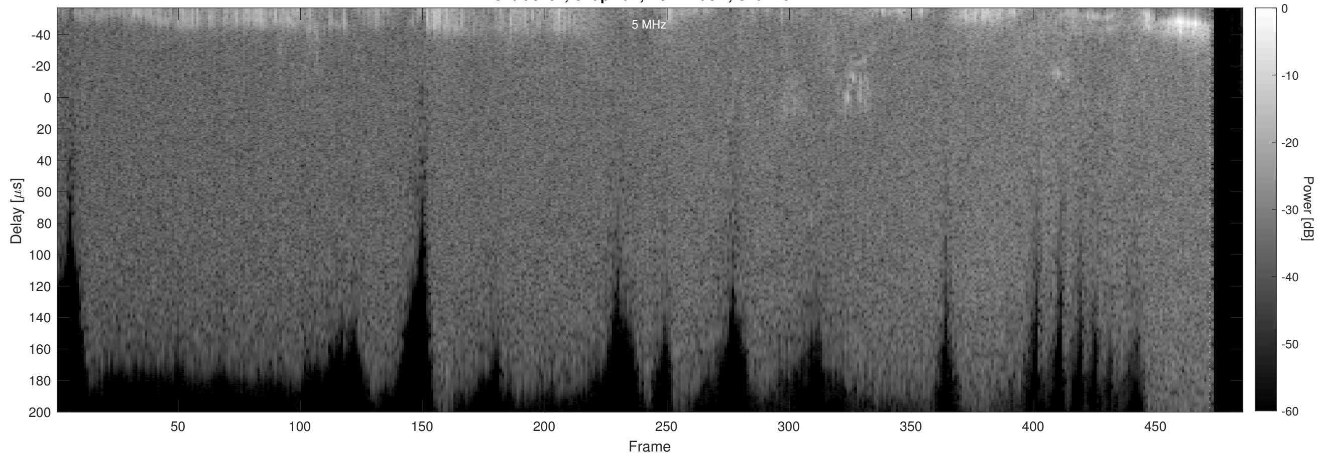
Orbit 3134, Chapman, No Window, Channel 2
