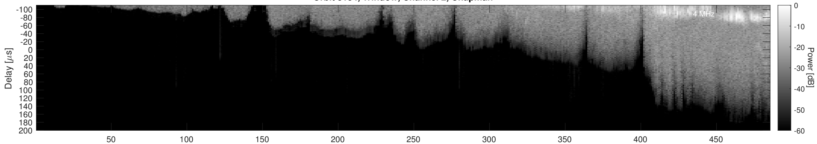
Orbit 3134, Window, Channel 2, Optimized
