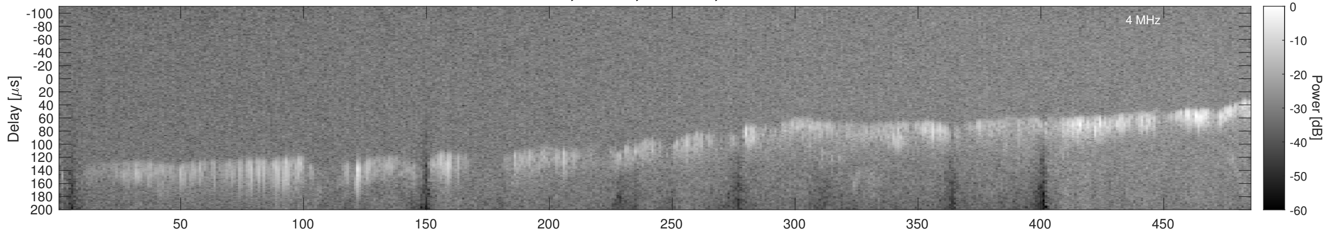
Orbit 3134, Window, Channel 2, Chapman
