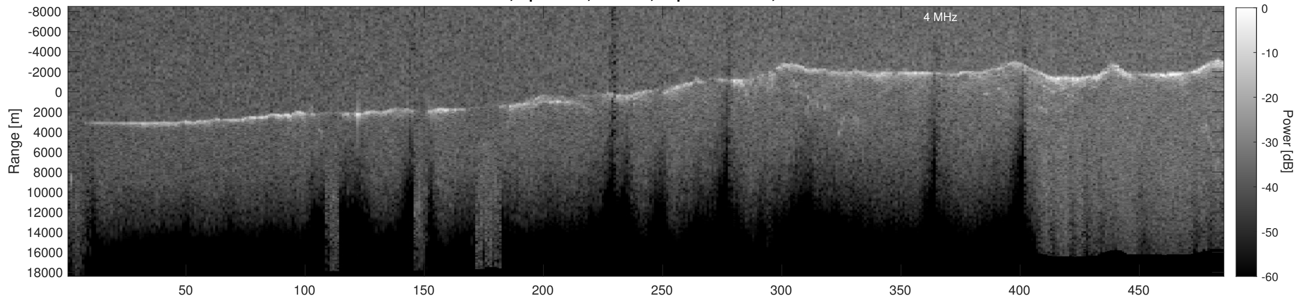
Orbit 3134, Depth-Corrected Cluttergram
