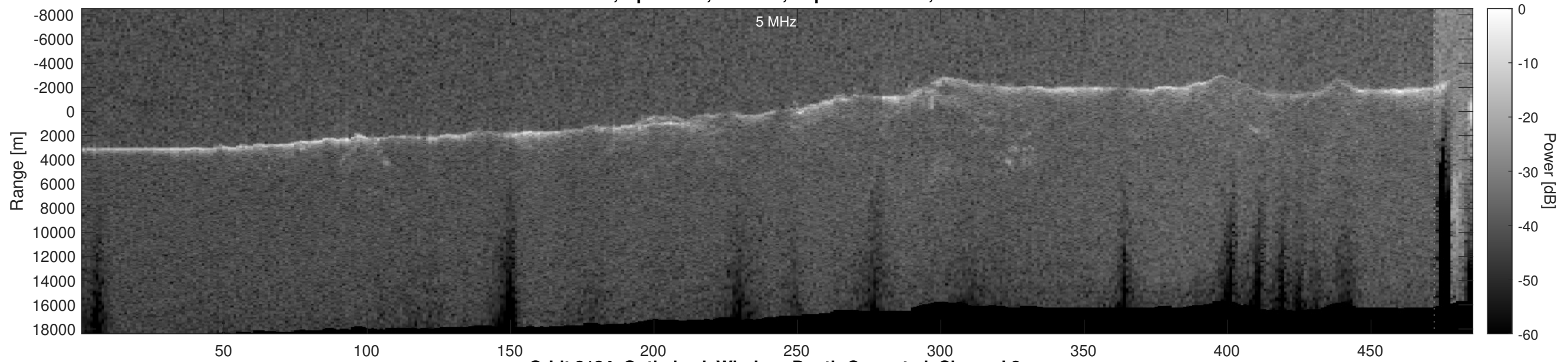
Orbit 3134, Optimized, Window, Depth-Corrected, Channel 2
