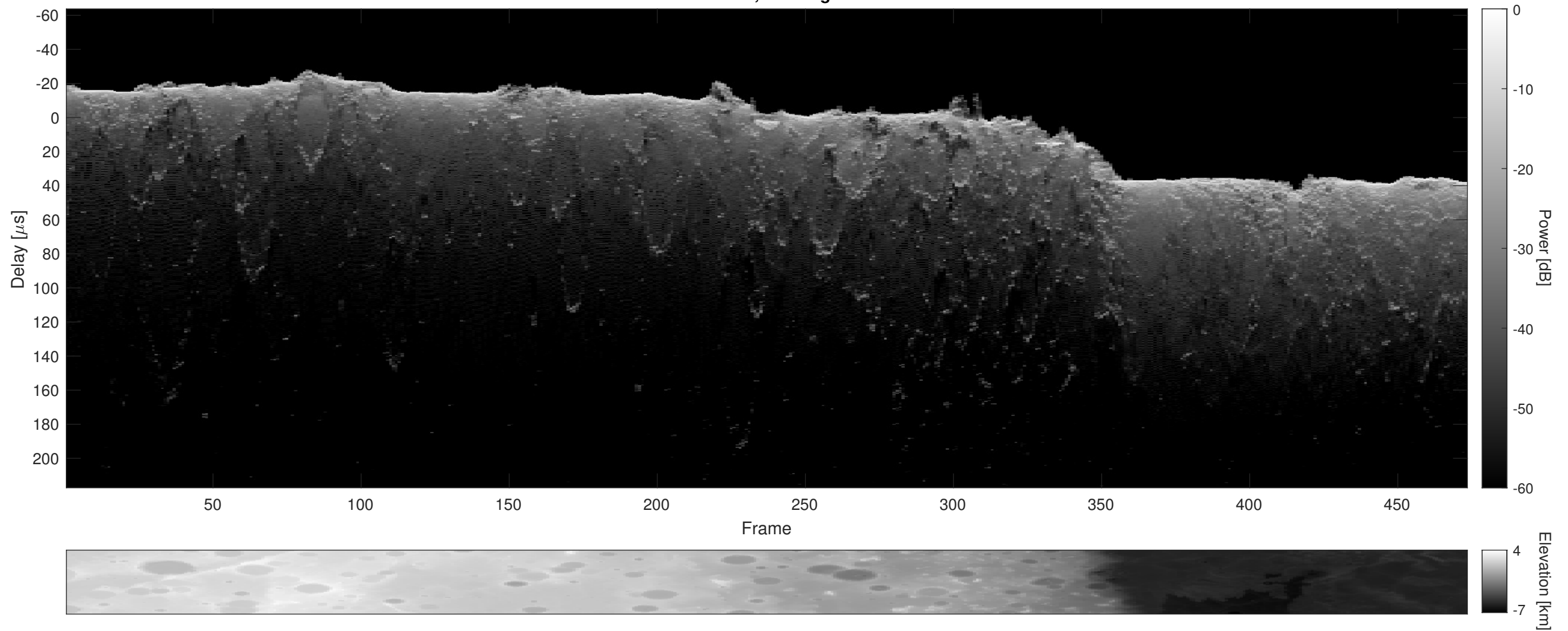
Orbit 3135, Cluttergram
